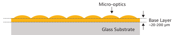
Polymer-on-glass Diffuser
