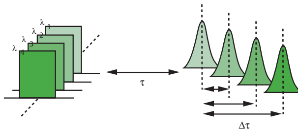
Chromatic Dispersion (CD)
