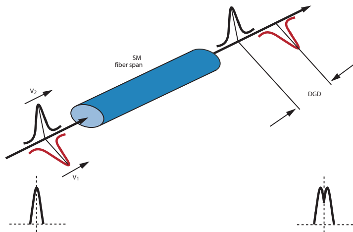
Polarization Mode Dispersion (PMD)
