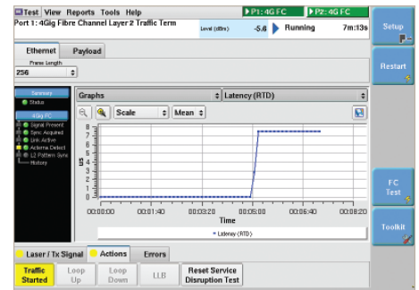
RTD Verification
