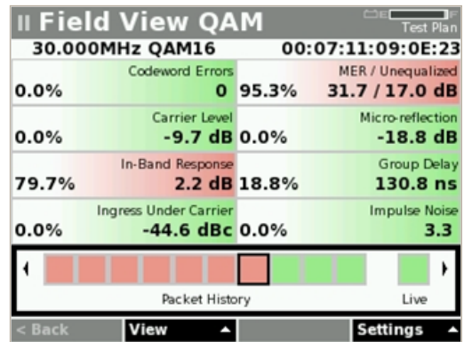
DSAM Field View QAM
