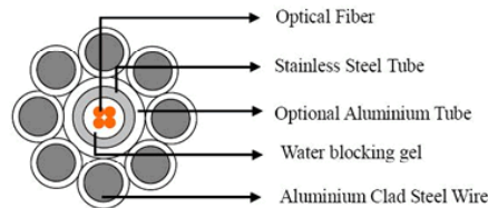
Central Loose Tube Type
