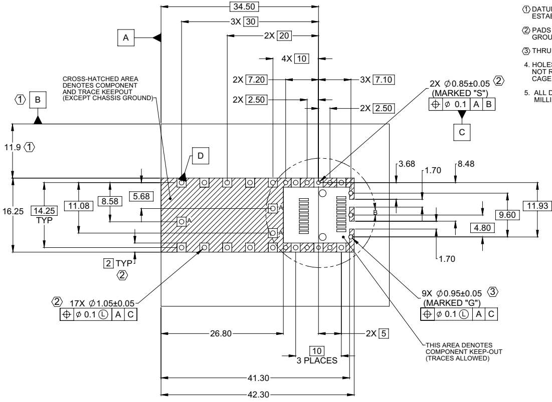
Figure 11 Double sided board layout
