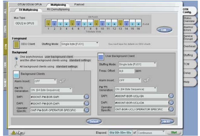
Figure 10: Multiplexing ODU2 in OPU3 using ONT-506 from JDSU
