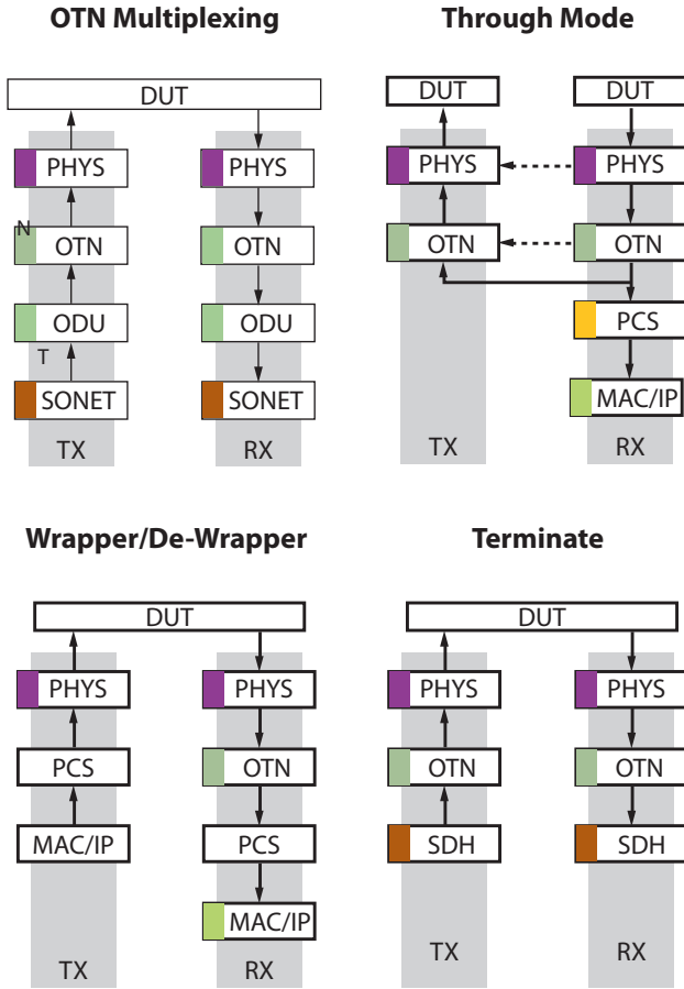
Figure 9: Test procedures for expanded transport structure acc. to ITU-T standard G.709 using test instrument ONT-506 of JDSU
