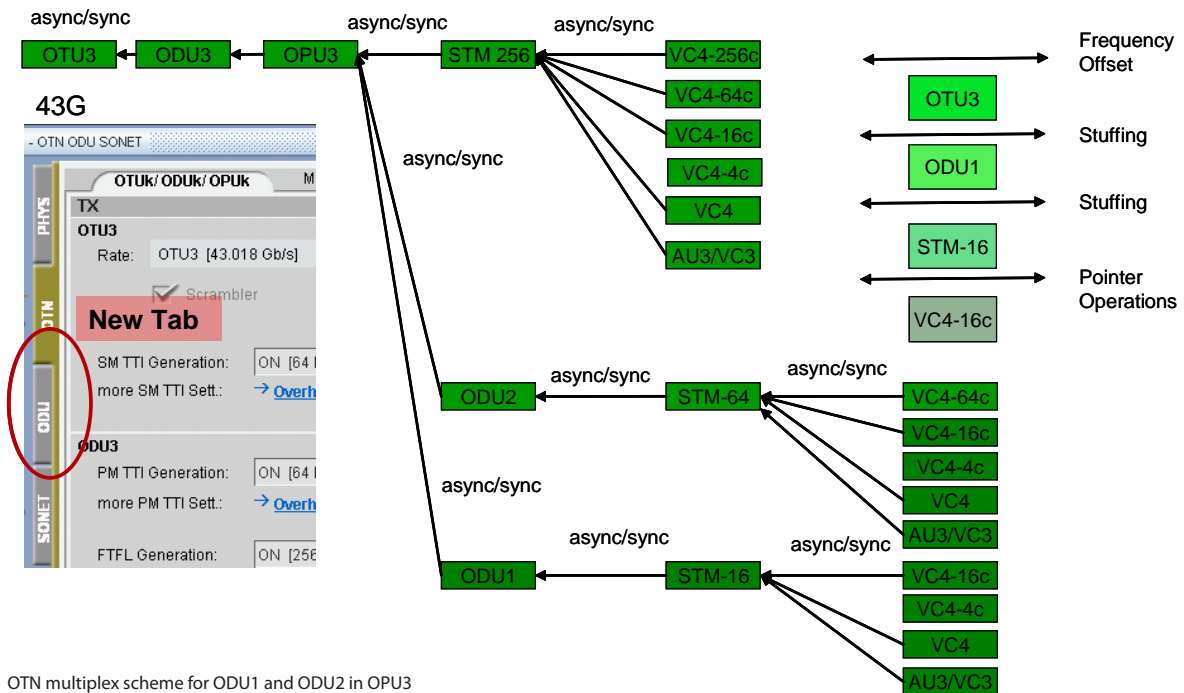
Figure 4 OTN multiplex scheme for ODU1 and ODU2 in OPU3
