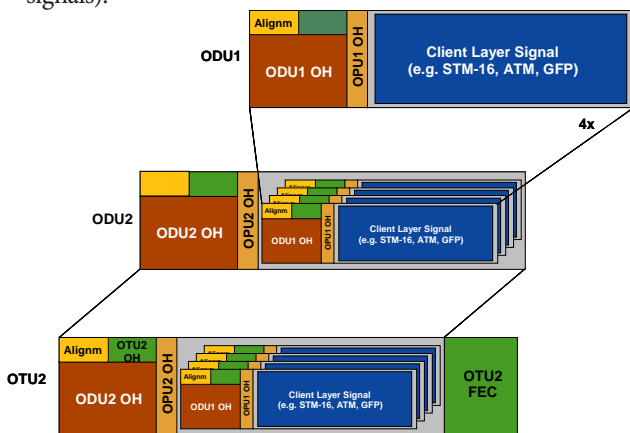
Figure 5: Multiplexing of ODU1 in OPU2 and OTU2 frames
