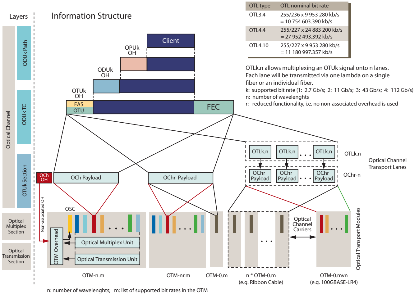
Figure 2: OTN signal structure according to ITU-T Recommendation G.709
