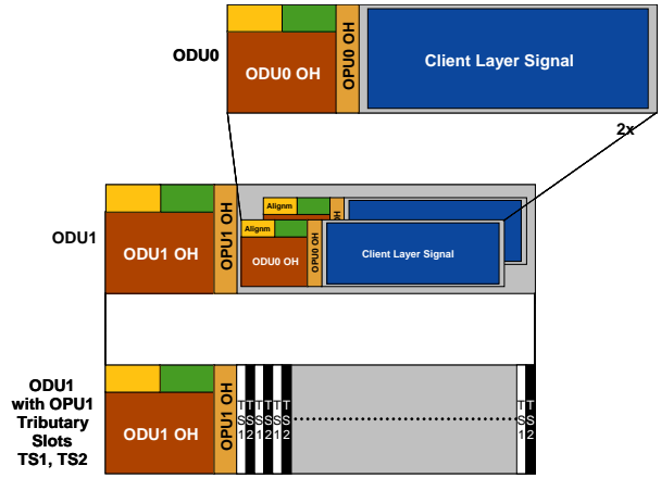
Figure 6 ODU0 frame for 1 Gigabit Ethernet source signal, multiplexed in OPU1 Further existing methods are listed in the ITU document G.Sup43 [2] by way of an appraisal. It remains to be seen which of these will be included in the standardization. Figure 7 shows the possible mapping structures for OTN with the various types of ODU multiplexing. Not all of these will be implemented. Experience will demonstrate which ones will be found most acceptable by the network providers.
