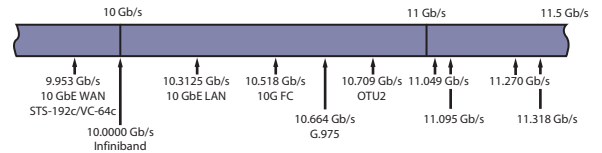
Structure of ODU1 and ODU2
