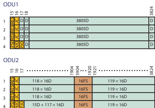
Figure 3: Variants at 10 Gbps and multiplex schemes
