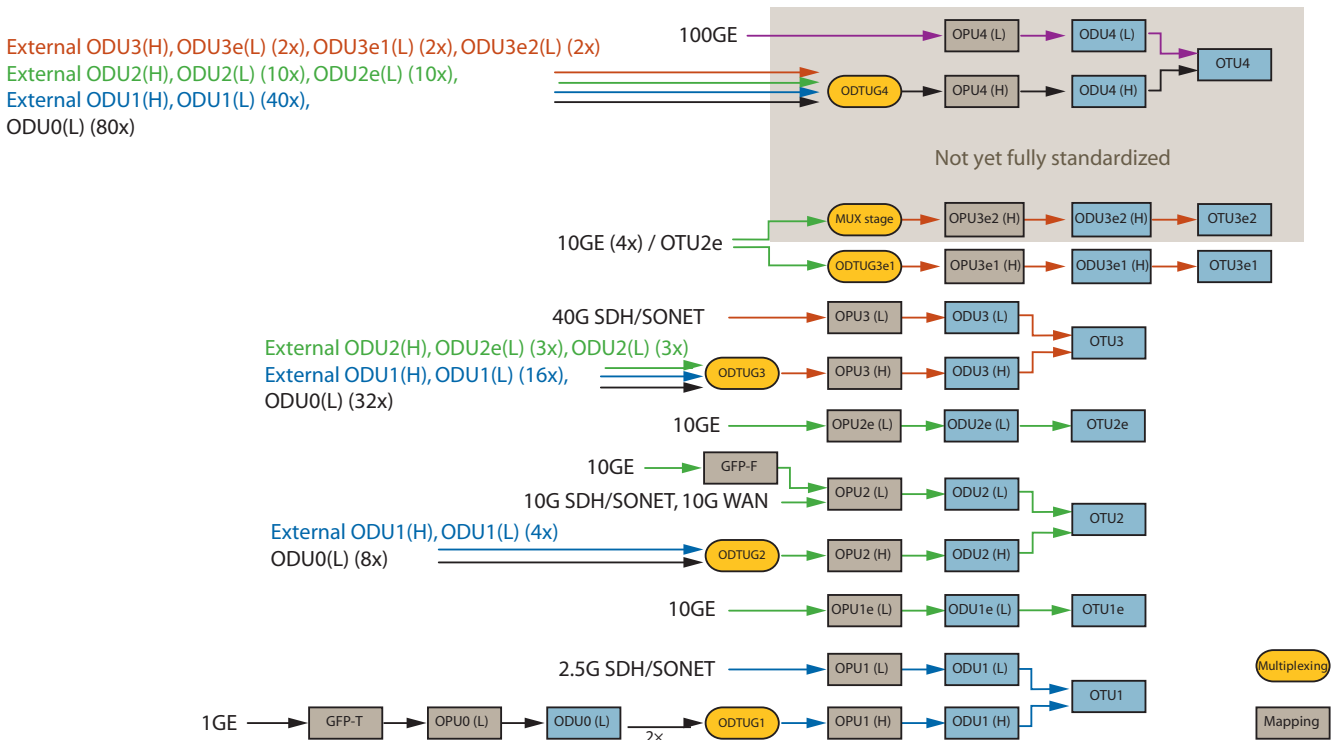
Figure 7: OTN mapping overview
