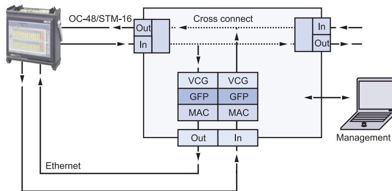
Figure 6: Interworking test using the JDSU ONT-503
