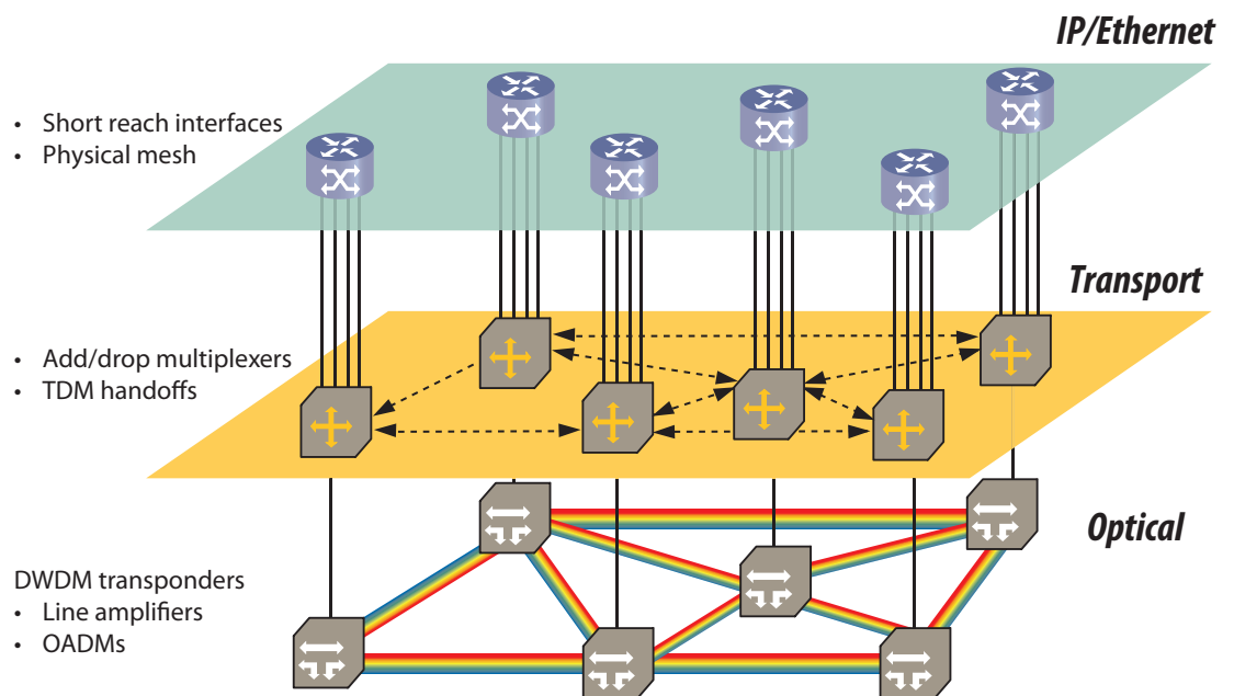
Figure 1. Multi-Layered Network
