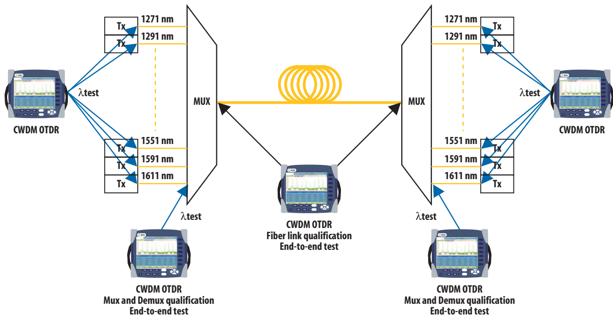
Figure 1 Evolution of a CWDM network
