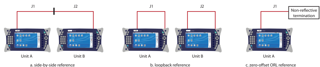
Figure 1. Reference procedures for side-by-side (a), loopback (b), and zero-offset ORL reference (c)
