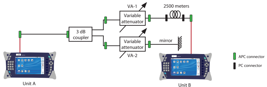
Figure 3. Calibrated link for experimental validation
