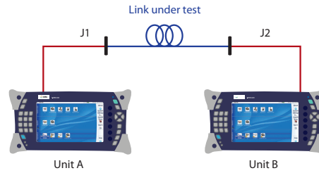
Figure 2. Experimental procedure for IL and ORL measurement of the link under test using the tool set
