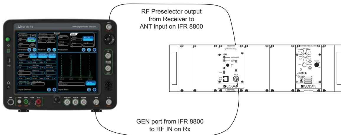
Figure G-13: Receiver RF Preselector Tuning
