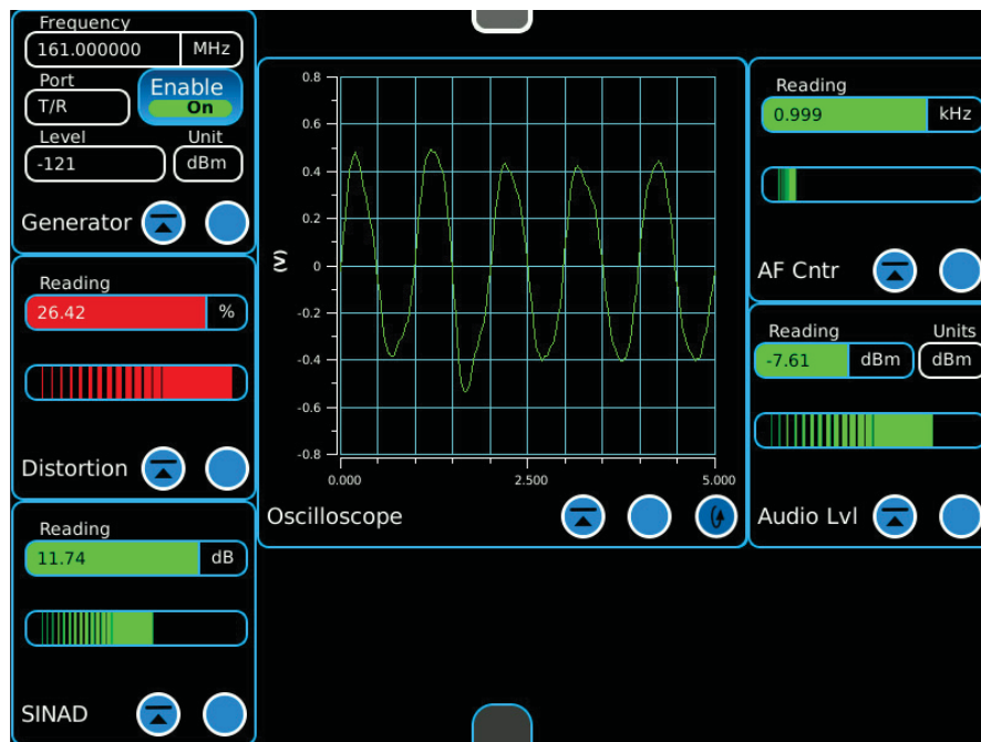
Figure G-8: Receiver Reference Sensitivity Measurement
