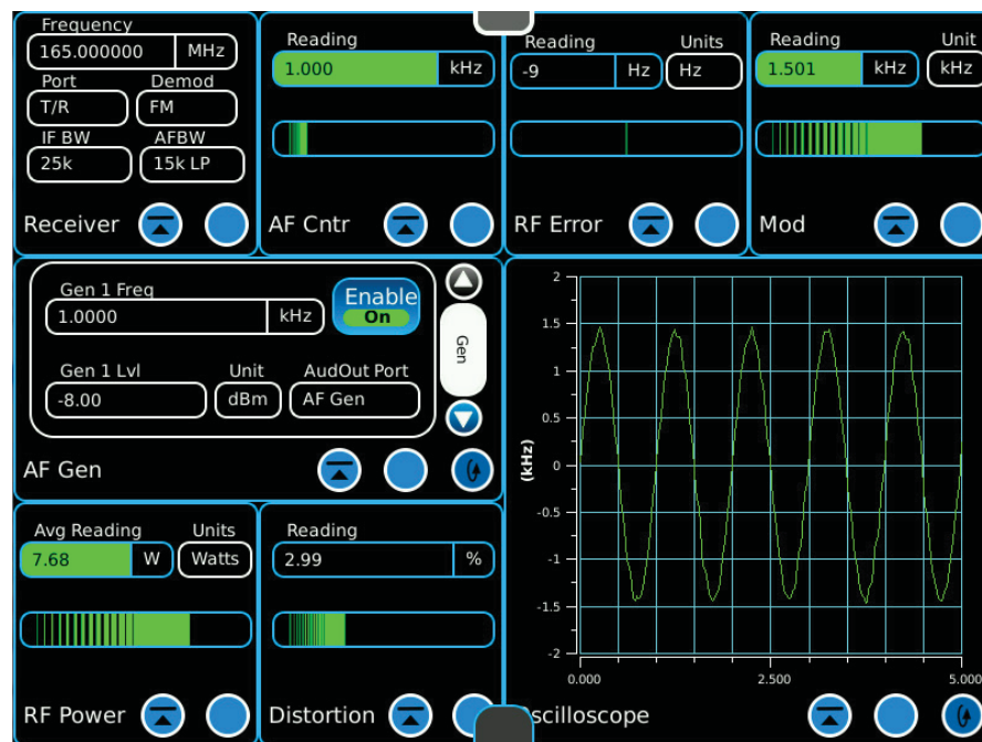
Figure G-24: Transmitter Deviation Measurement
