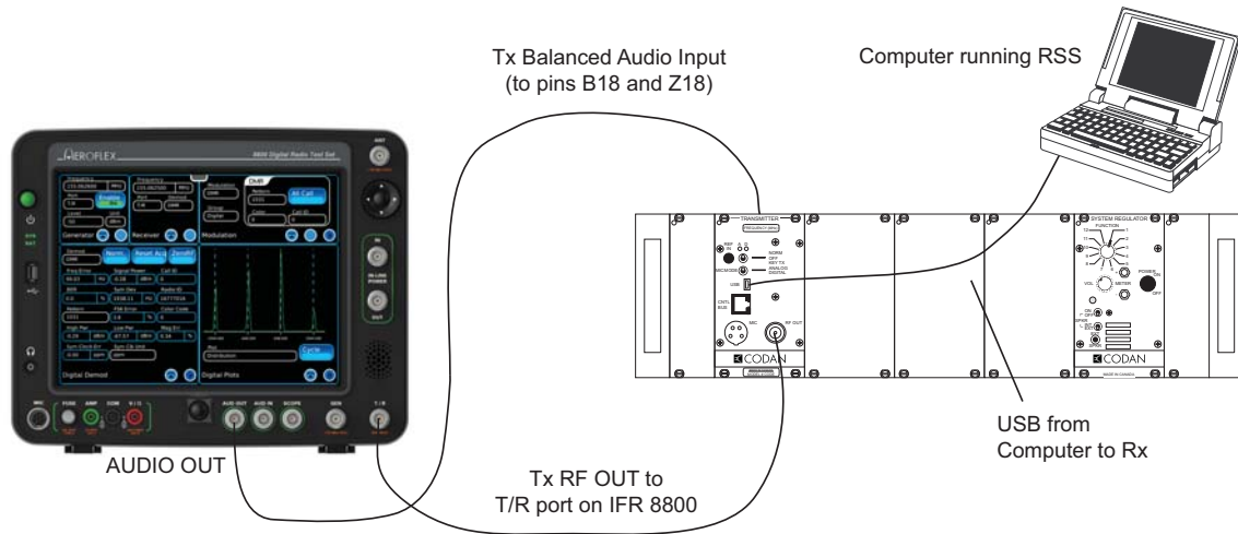
Figure G-30: Transmitter Digital Testing
