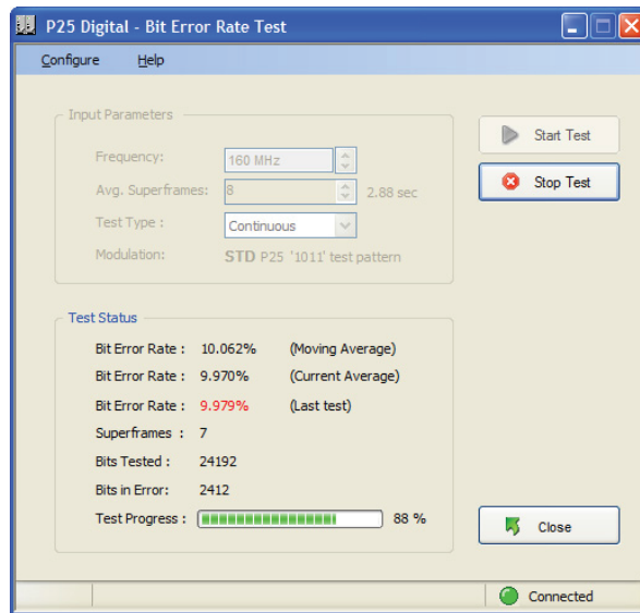
Figure G-12: RSS Receiver Bit Error Rate Test
