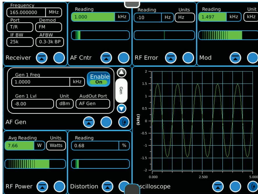
Figure G-22: Tx Distortion and Power Measurements
