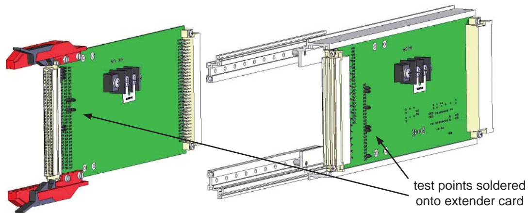
Figure G-2: EC-96D1 and EC-48RD Direct Connect Extender Cards with Test Points Added
