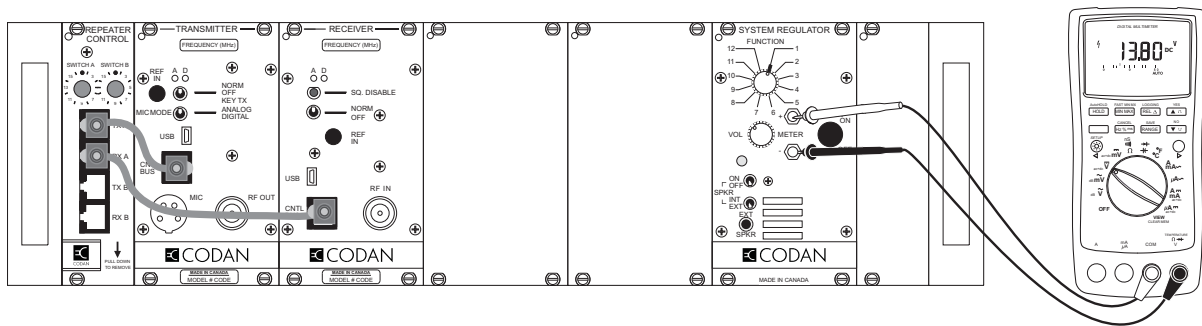
Figure G-3: System Regulator Voltage Testing
