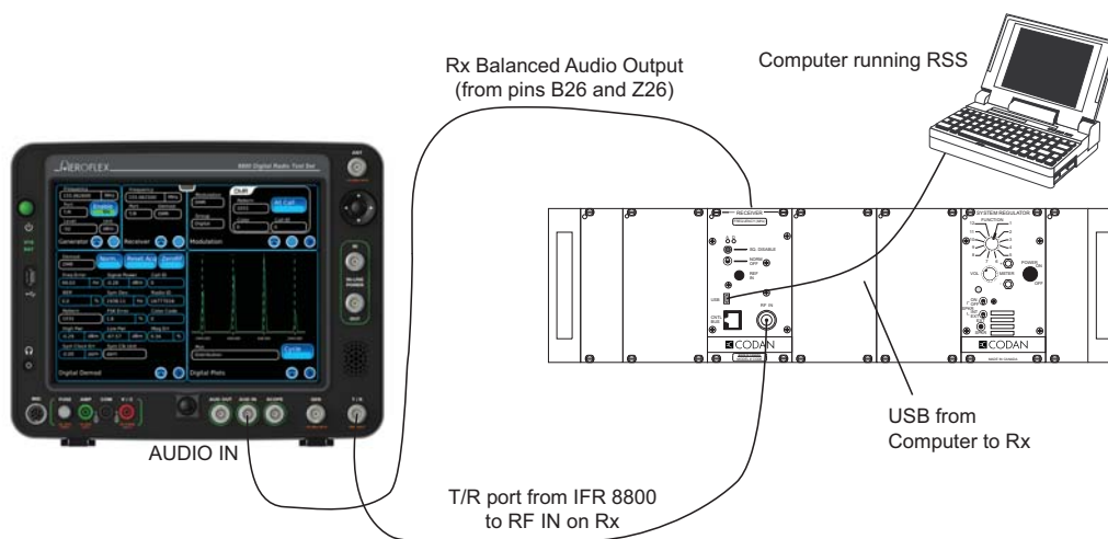
Figure G-10: Receiver Digital Testing
