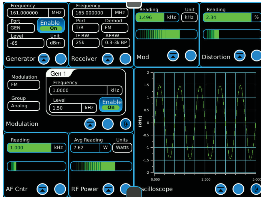
Figure G-34: System Analog Duplex Measurement
