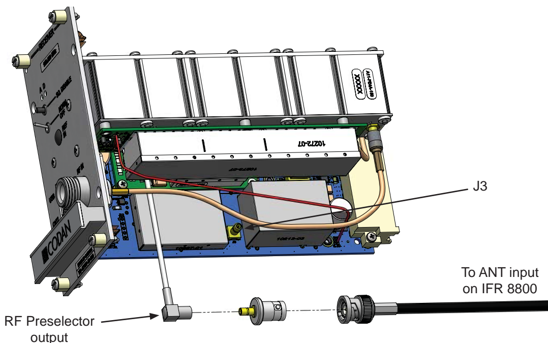
Figure G-14: Receiver RF Preselector Connection
