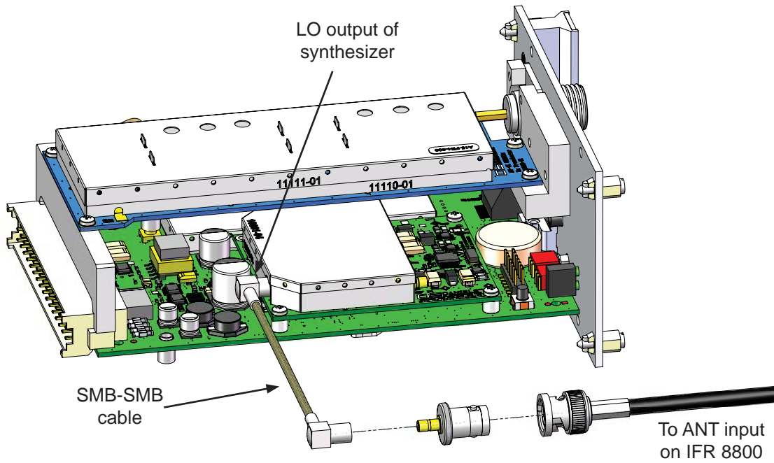
Figure G-18: UHF 700 / 800 / 900 MHz Receiver Reference Oscillator Connection
