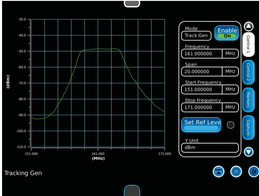
Figure G-15: Receiver RF Preselector
