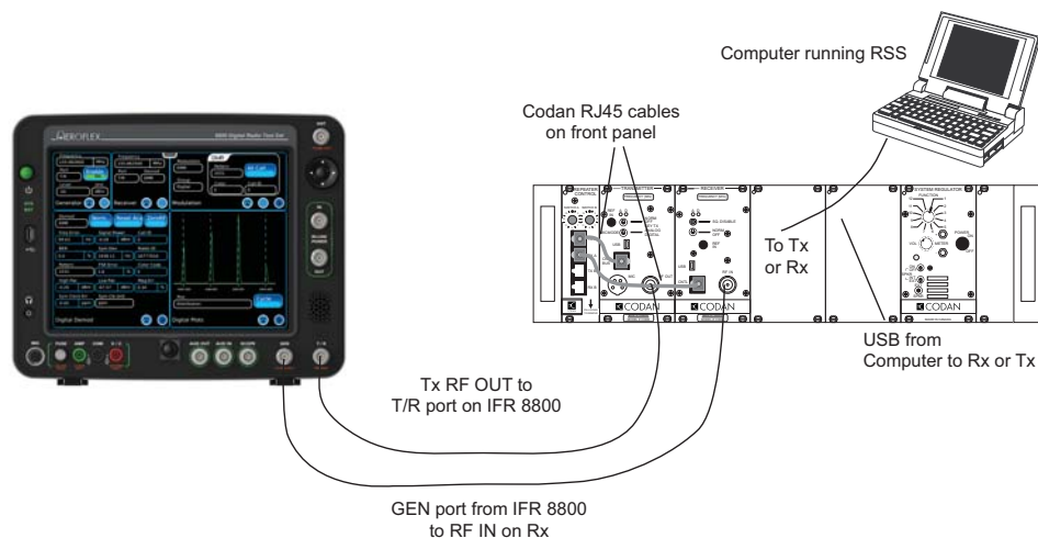
Figure G-36: System Duplex Digital Testing
