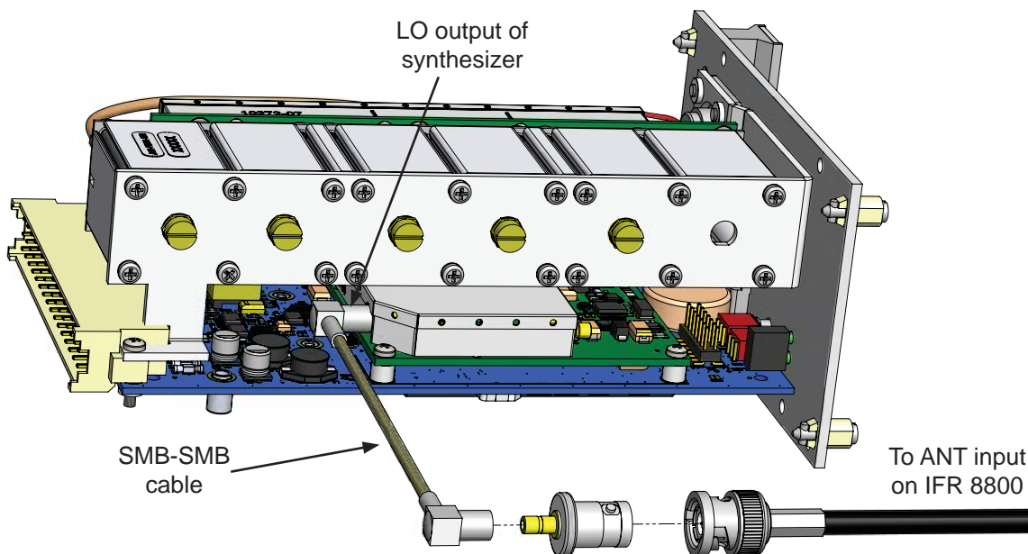
Figure G-17: VHF and UHF 400 MHz Receiver Reference Oscillator Connection
