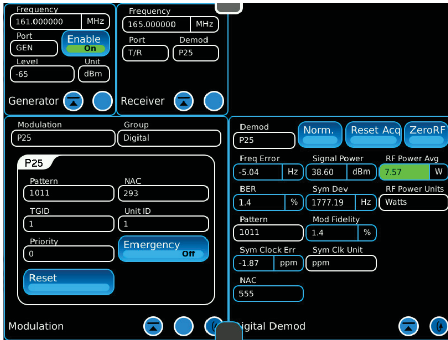
Figure G-37: System Digital Duplex Check
