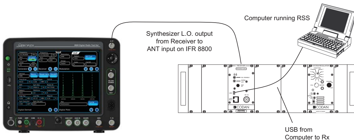
Figure G-16: Receiver Reference Oscillator Testing
