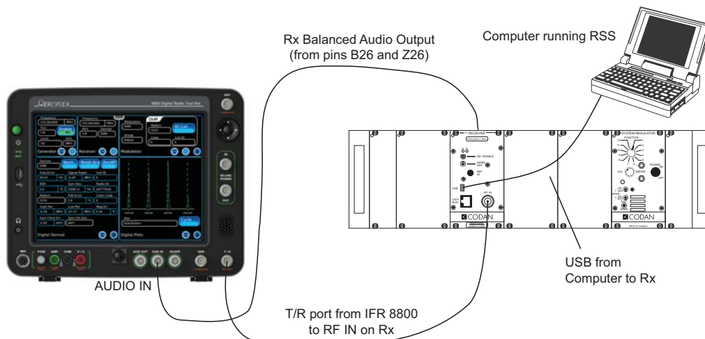
Figure G-4: Receiver Analog Testing
