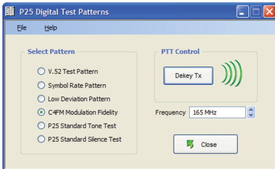
Figure G-32: RSS Transmitter Modulation Fidelity Test Pattern
