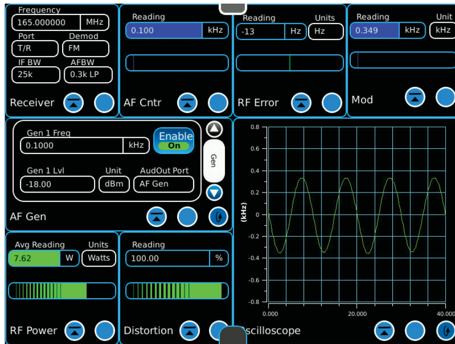
Figure F-28: Transmitter CTCSS Tone and Deviation Measurement
