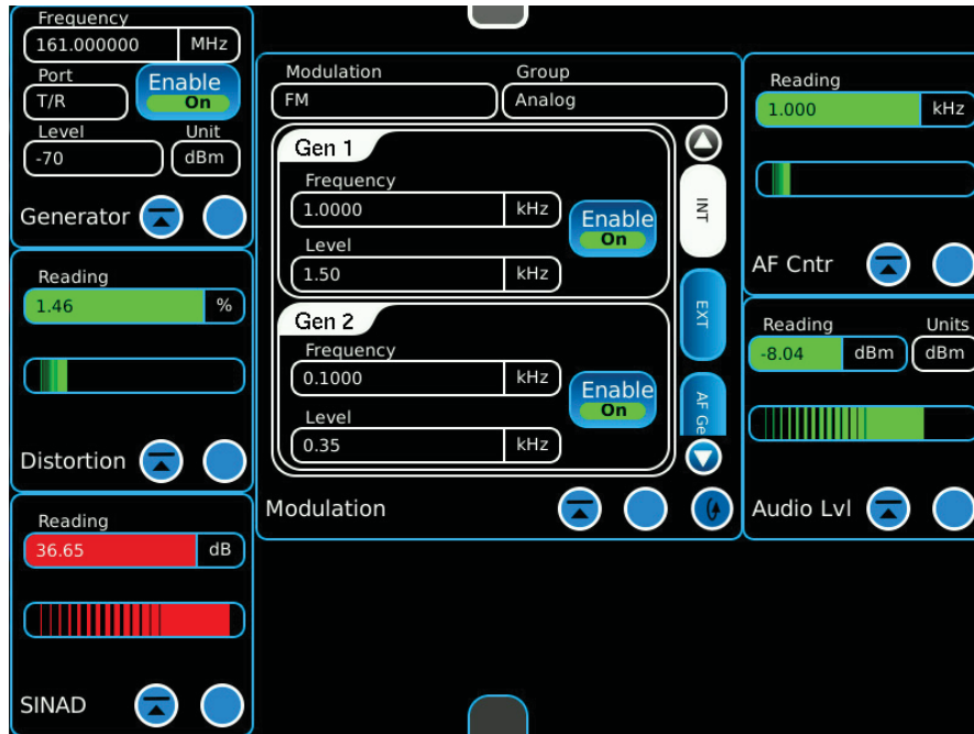
Figure G-6: Receiver Distortion Measurement
