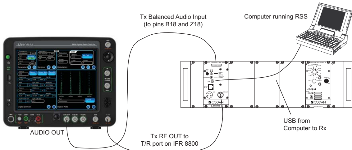
Figure G-21: Transmitter Analog Testing
