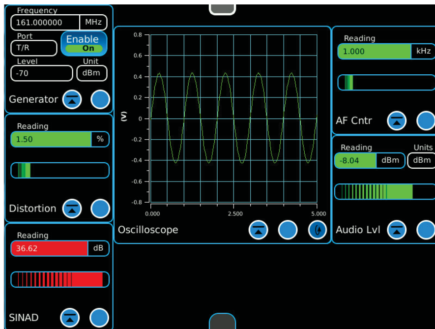
Figure G-7: Receiver Oscilloscope View
