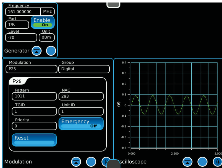
Figure G-11: Receiver Digital Check
