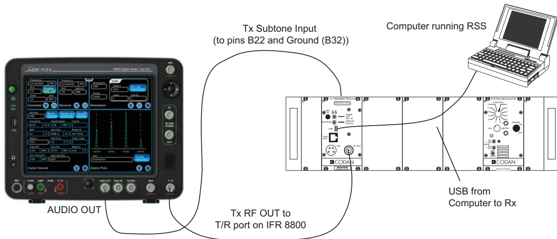
Figure G-27: Transmitter CTCSS Testing
