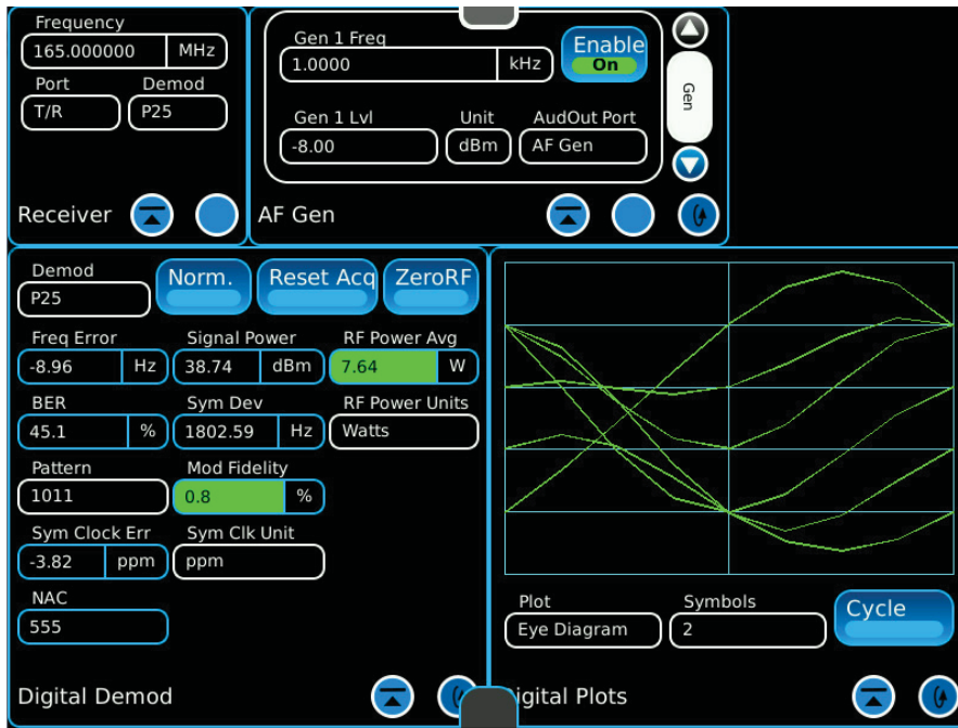
Figure G-31 Transmitter Digital Check
