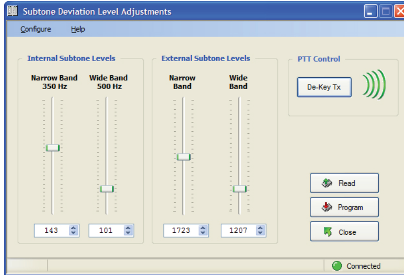
Figure G-29: RSS Transmitter Subtone Deviation Level Adjustment
