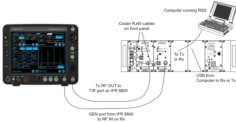
Figure G-33: System Duplex Analog Testing
