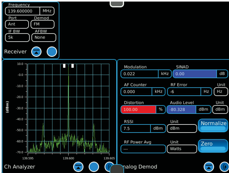
Figure G-19: Receiver Reference Oscillator Measurement
